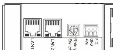
Wire Connection
