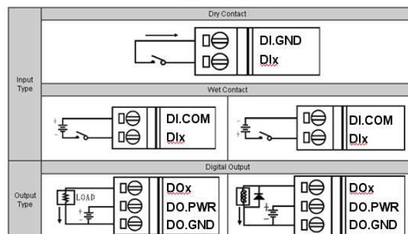
Wire Connection
